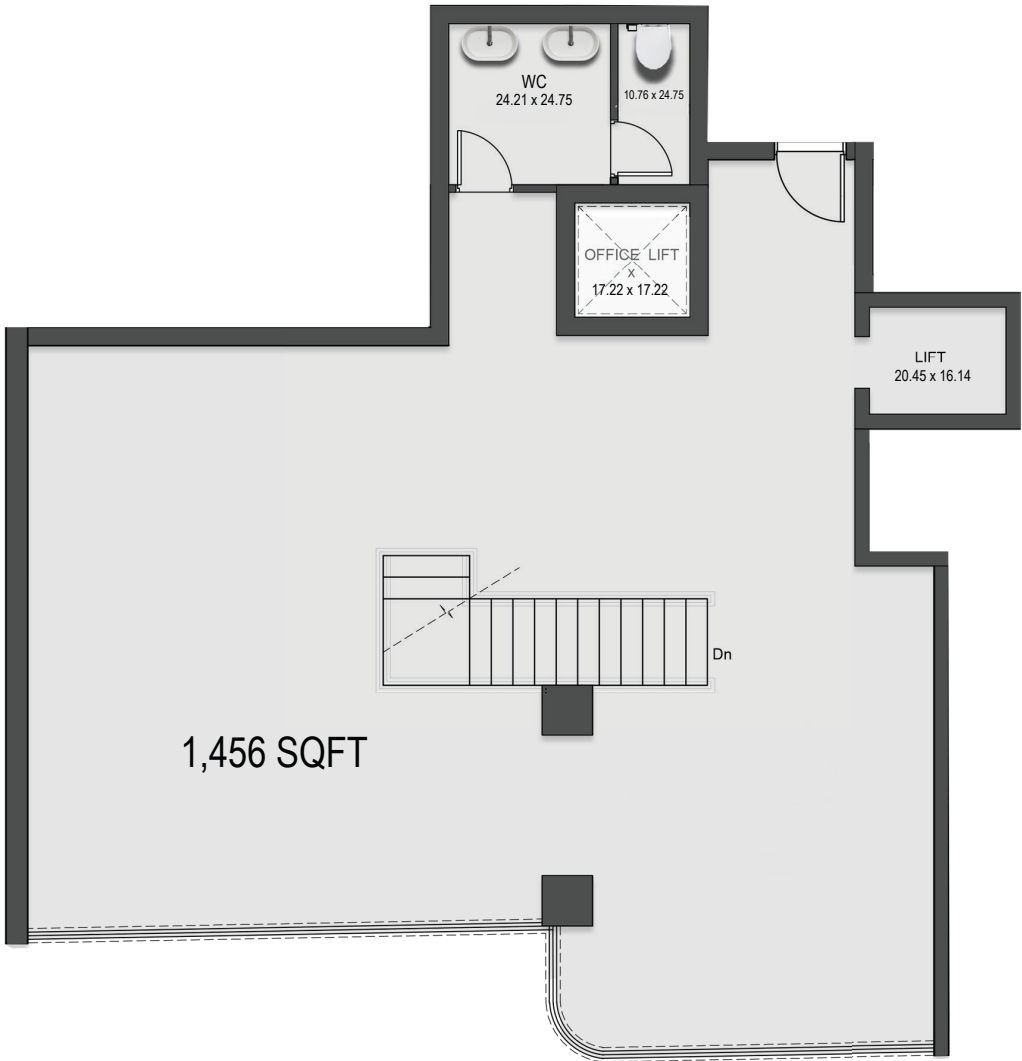
P1 FLOOR PLAN
