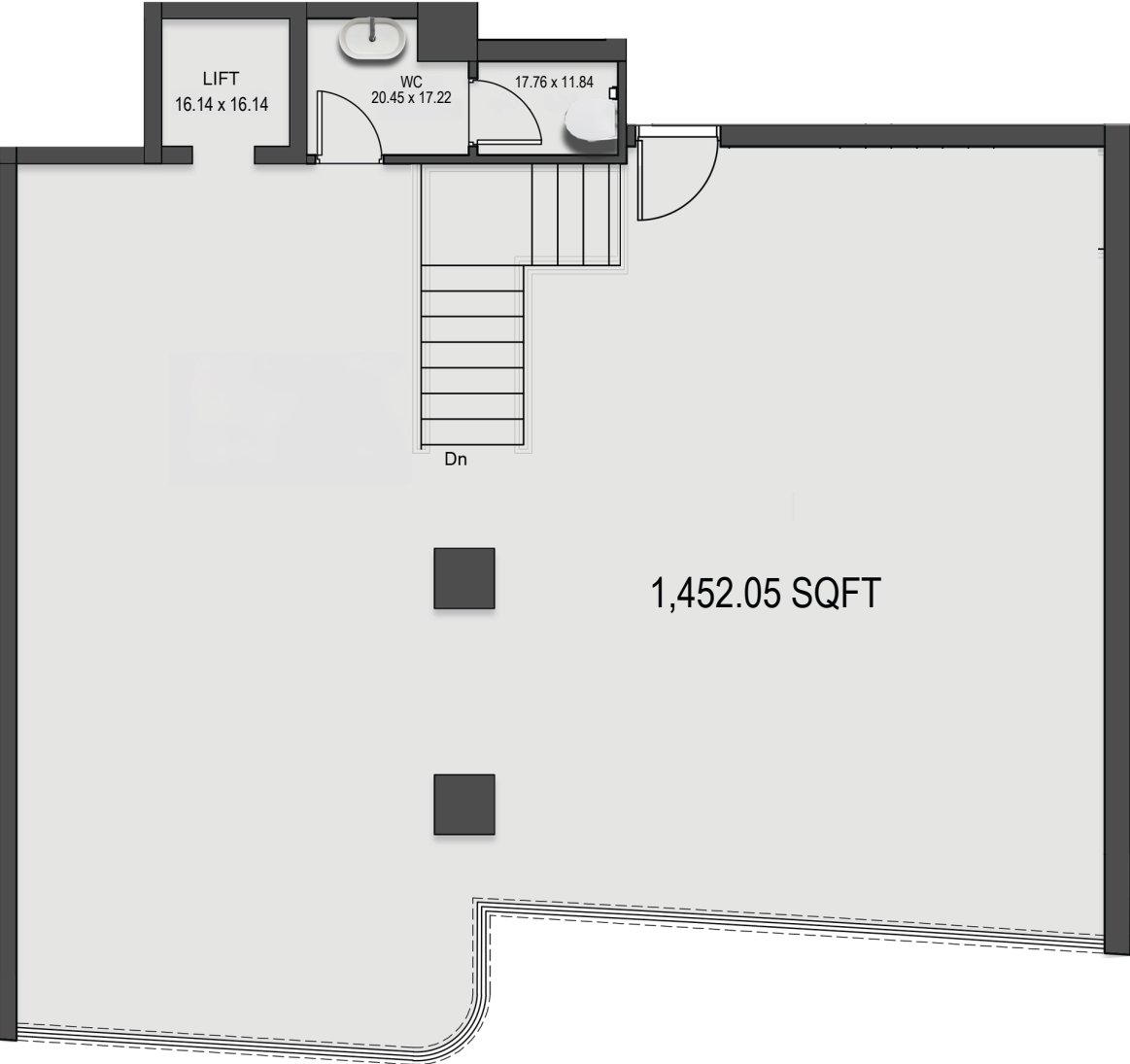
P1 FLOOR PLAN
