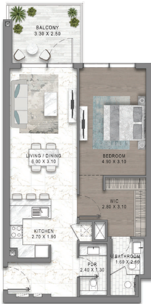
1BR - TYPE J2
