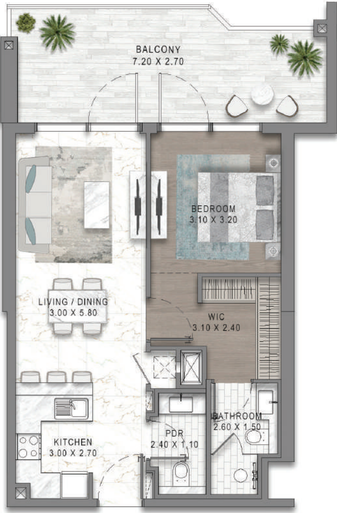
1BR - TYPE B12
