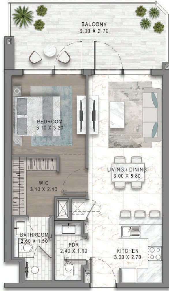
1BR - TYPE C5
