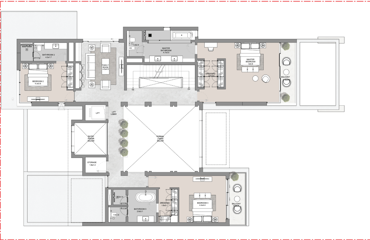
First Floor
