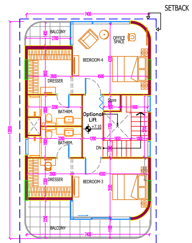
SECOND FLOOR
