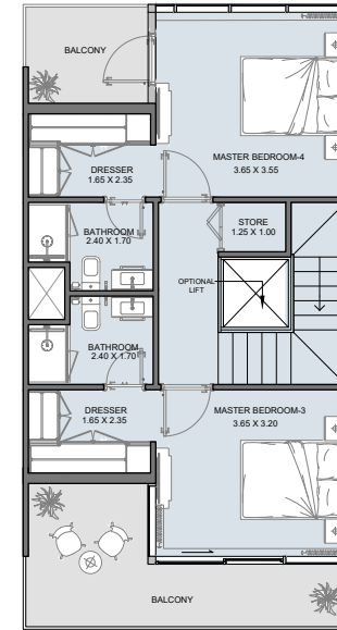
SECOND FLOOR Middle Unit
