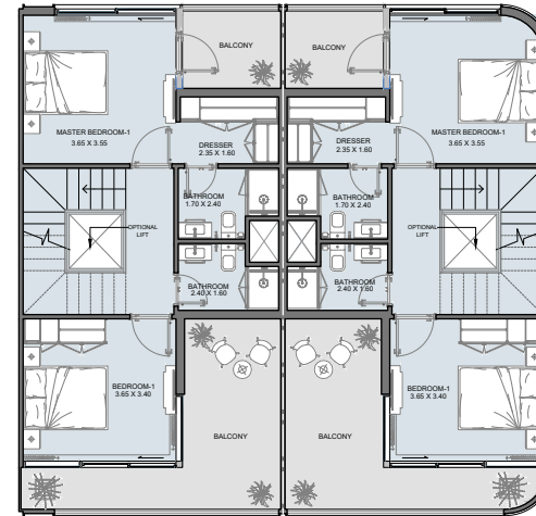
FIRST FLOOR Middle Unit
