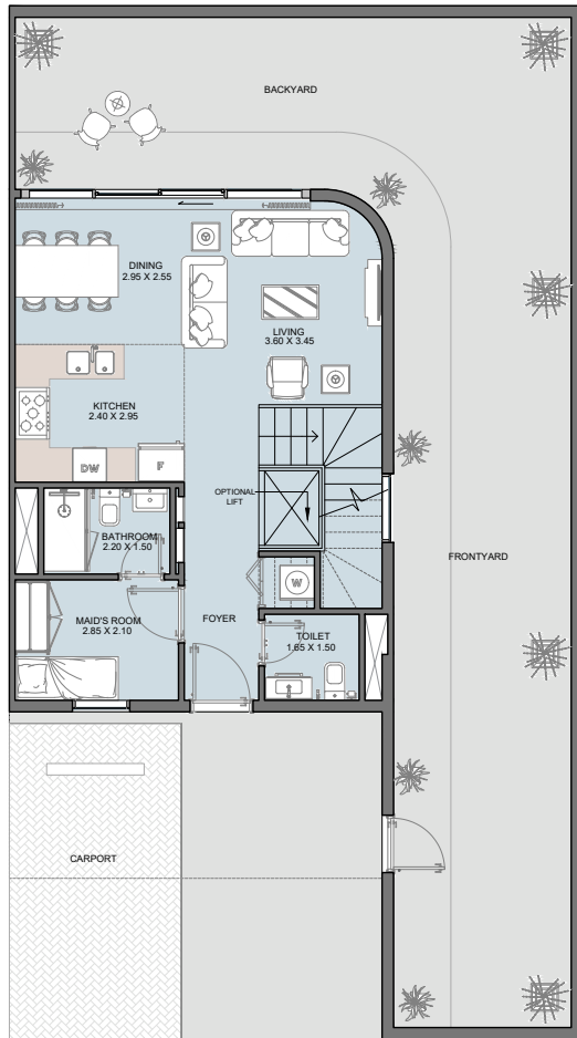
GROUND FLOOR Corner Unit
