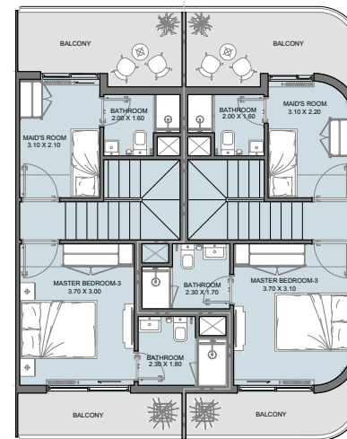
SECOND FLOOR Middle Unit
