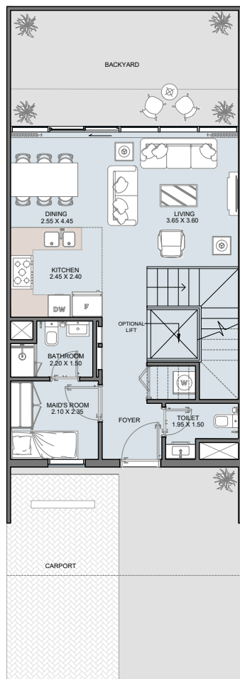
GROUND FLOOR Middle Unit
