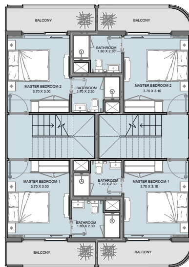
FIRST FLOOR Middle Unit
