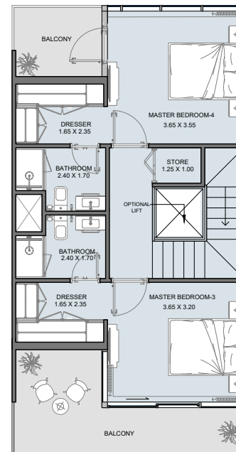
SECOND FLOOR Middle Unit
