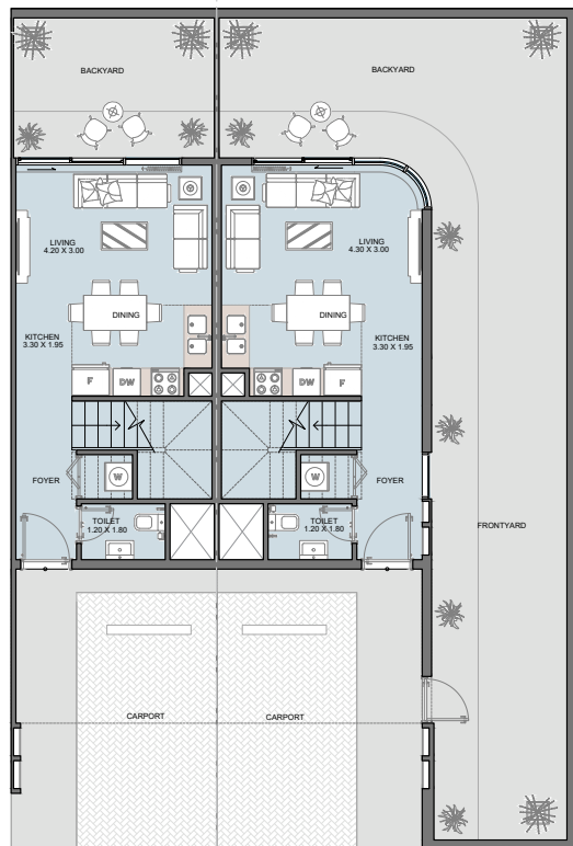
GROUND FLOOR Middle Unit
