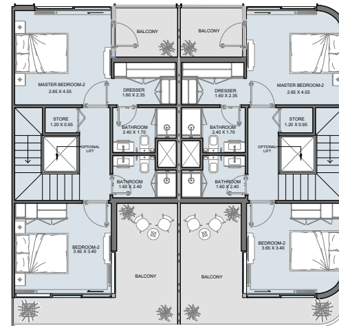
SECOND FLOOR Middle Unit
