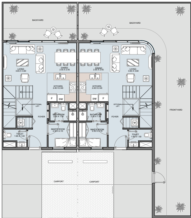
GROUND FLOOR Middle Unit
