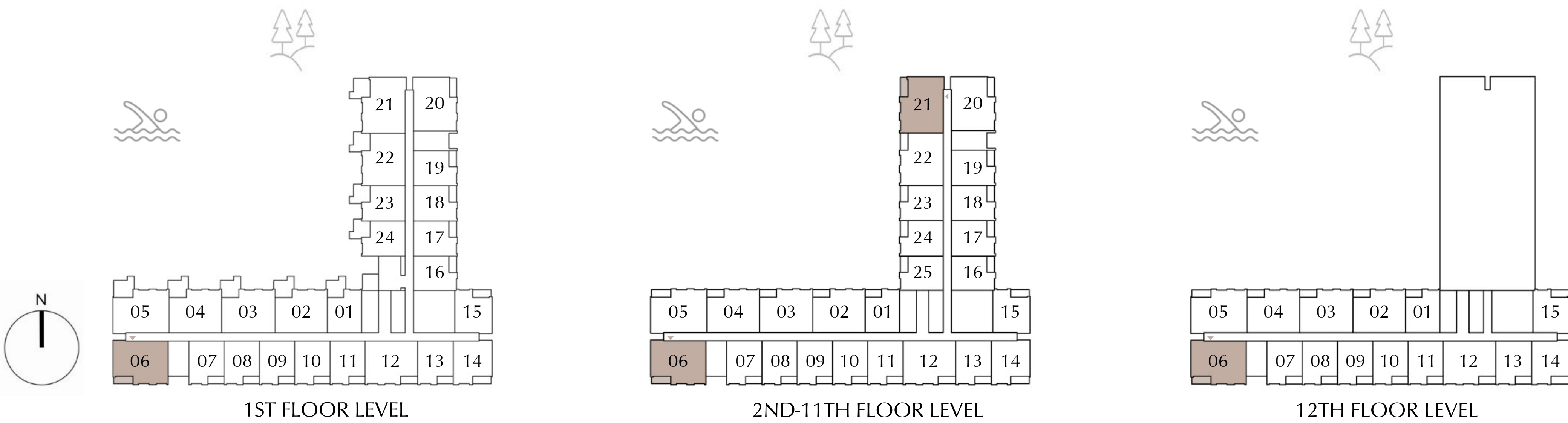
KEY PLAN
