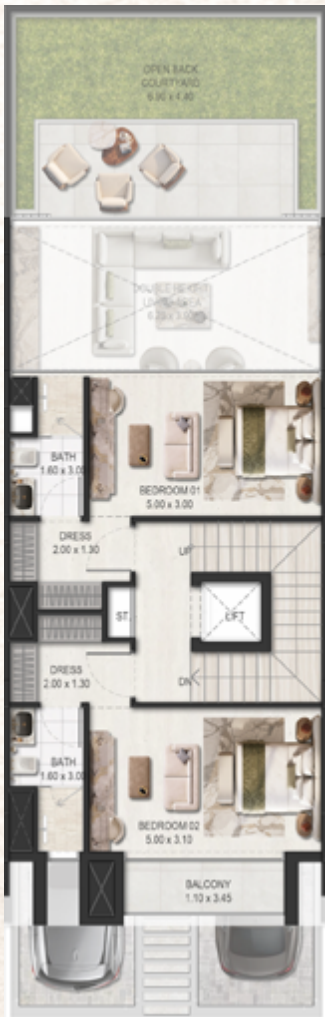
Mid Unit Villa (First floor)
