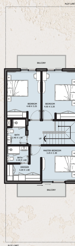
1ST FLOOR
