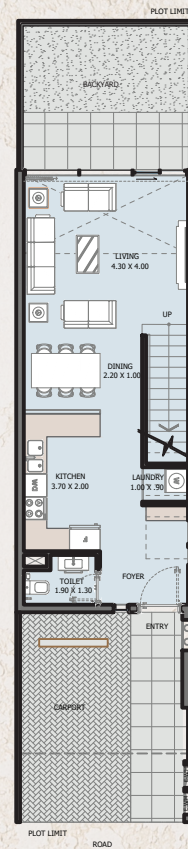
GROUND FLOOR
