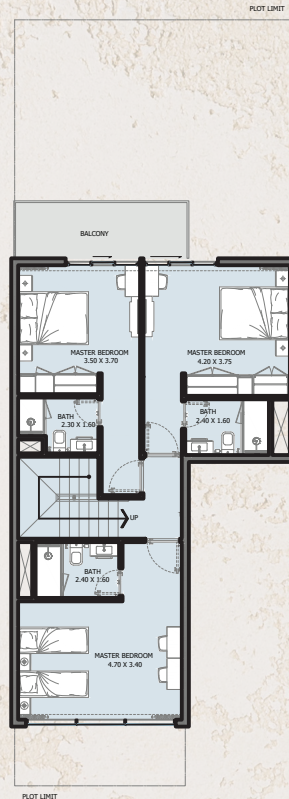
1ST FLOOR
