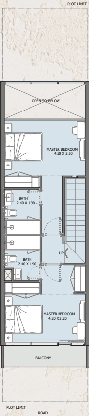
1ST FLOOR
