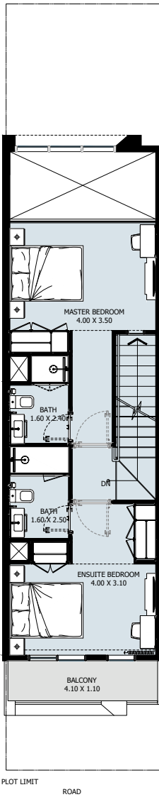
1ST FLOOR
