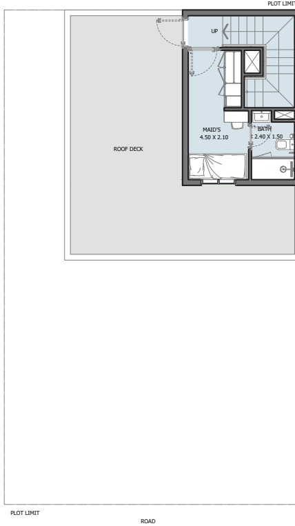
2ND FLOOR
