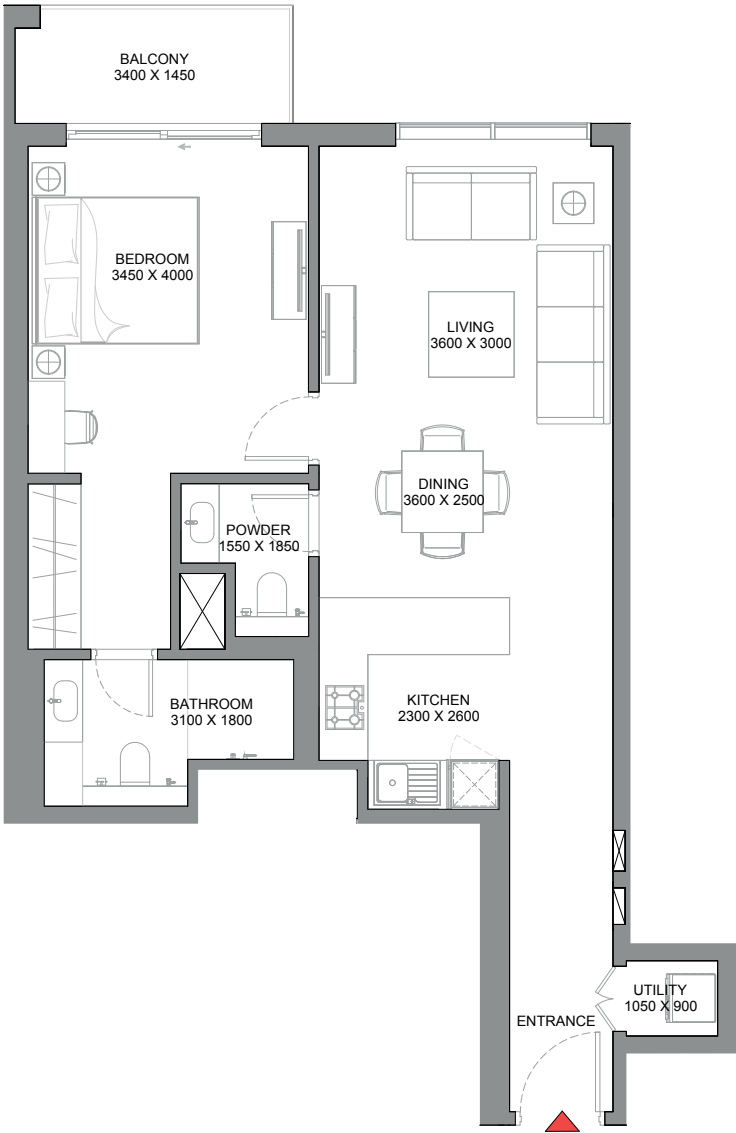
TYPICAL LEVEL 07-17, 21-30, 33-42, 46-55
