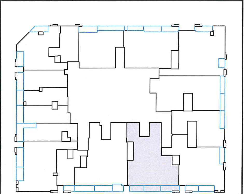
TYPICAL FLOOR PLAN ( 2-26 )
