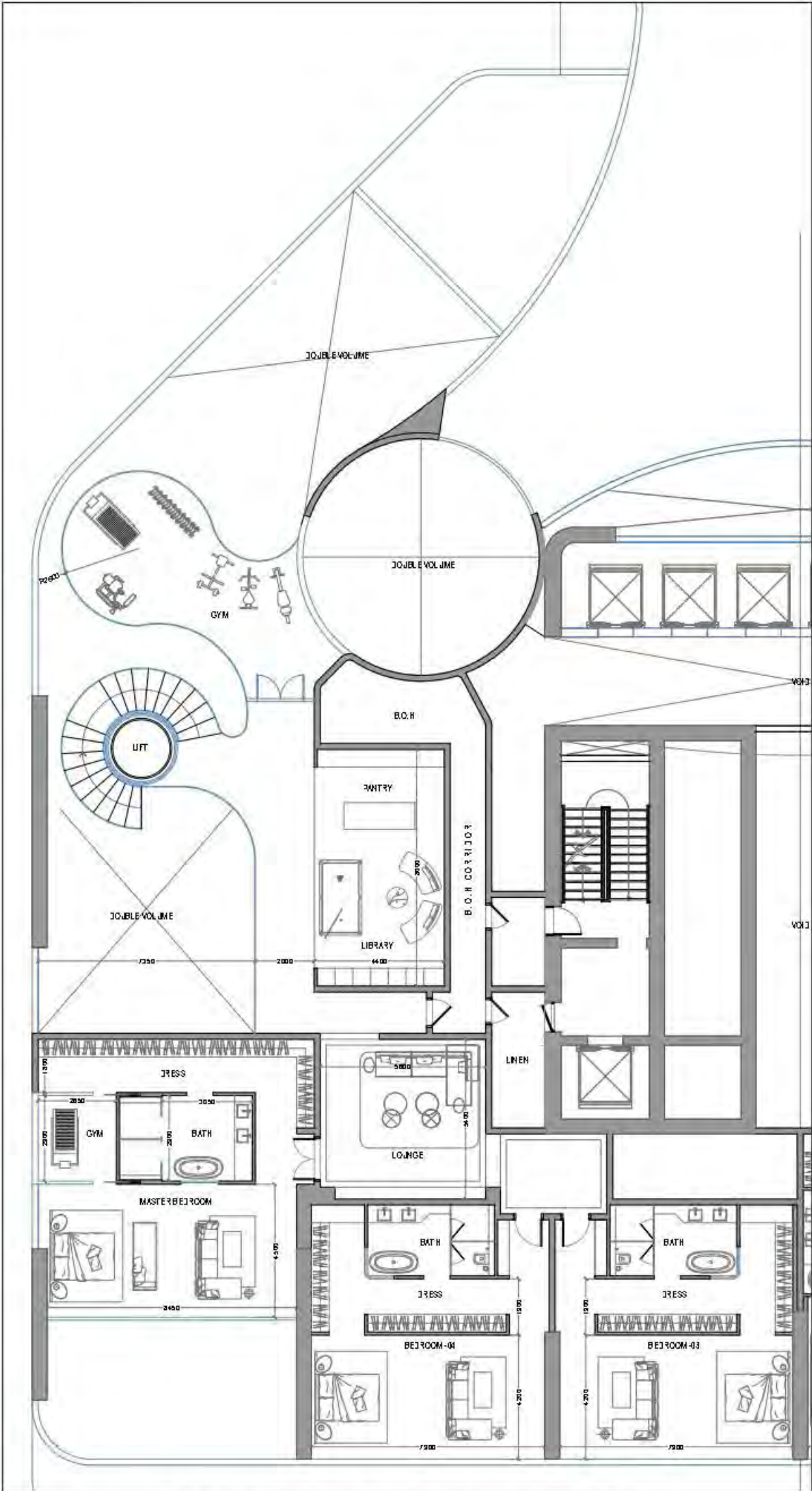
UPPER LEVEL PLAN
