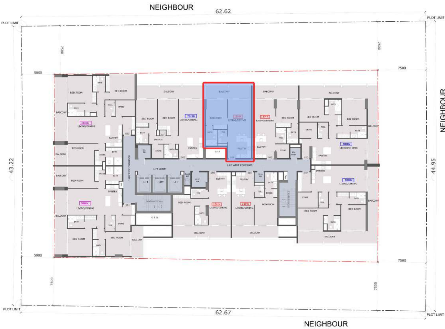
KEY PLAN
