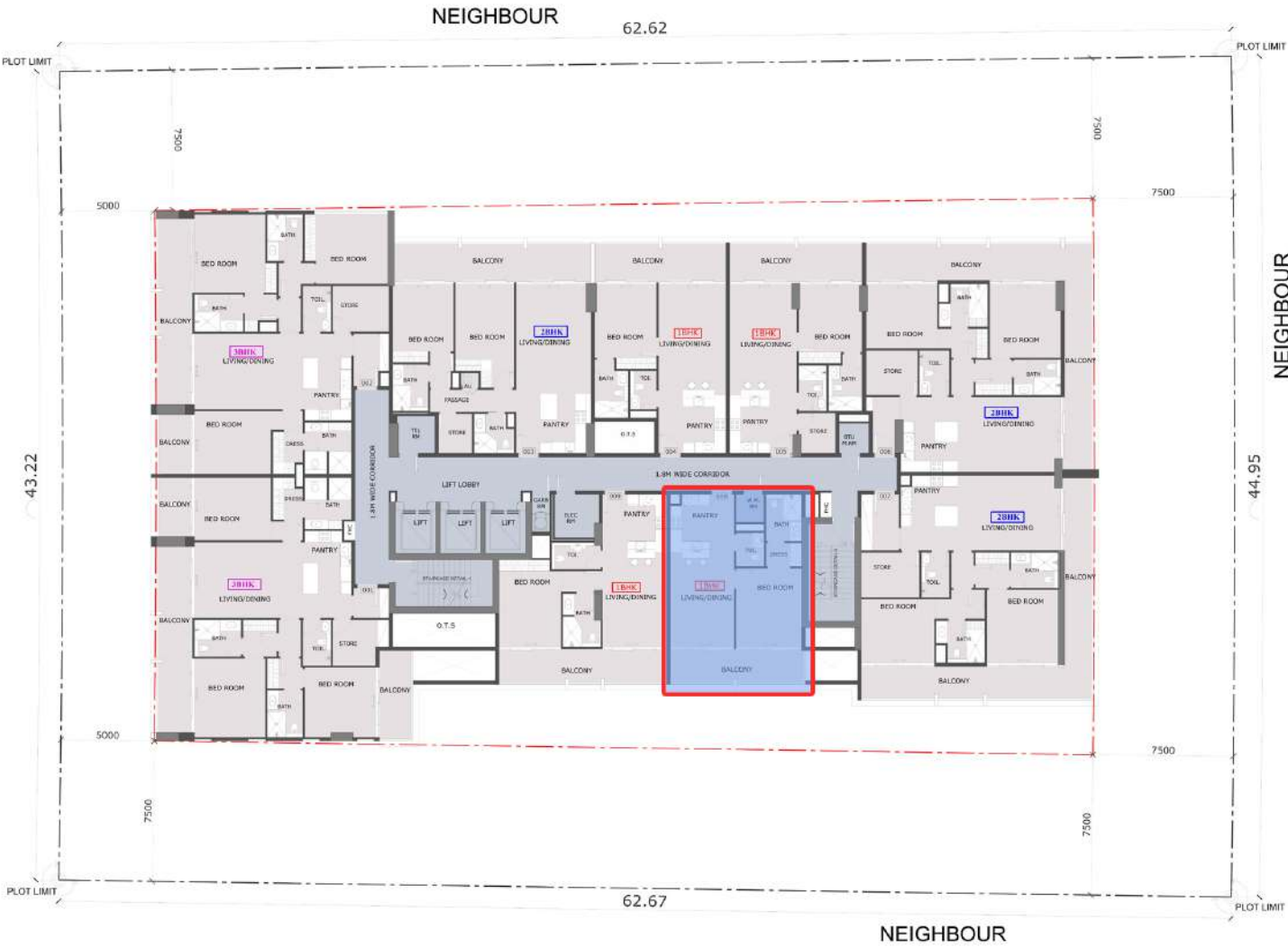
KEY PLAN
