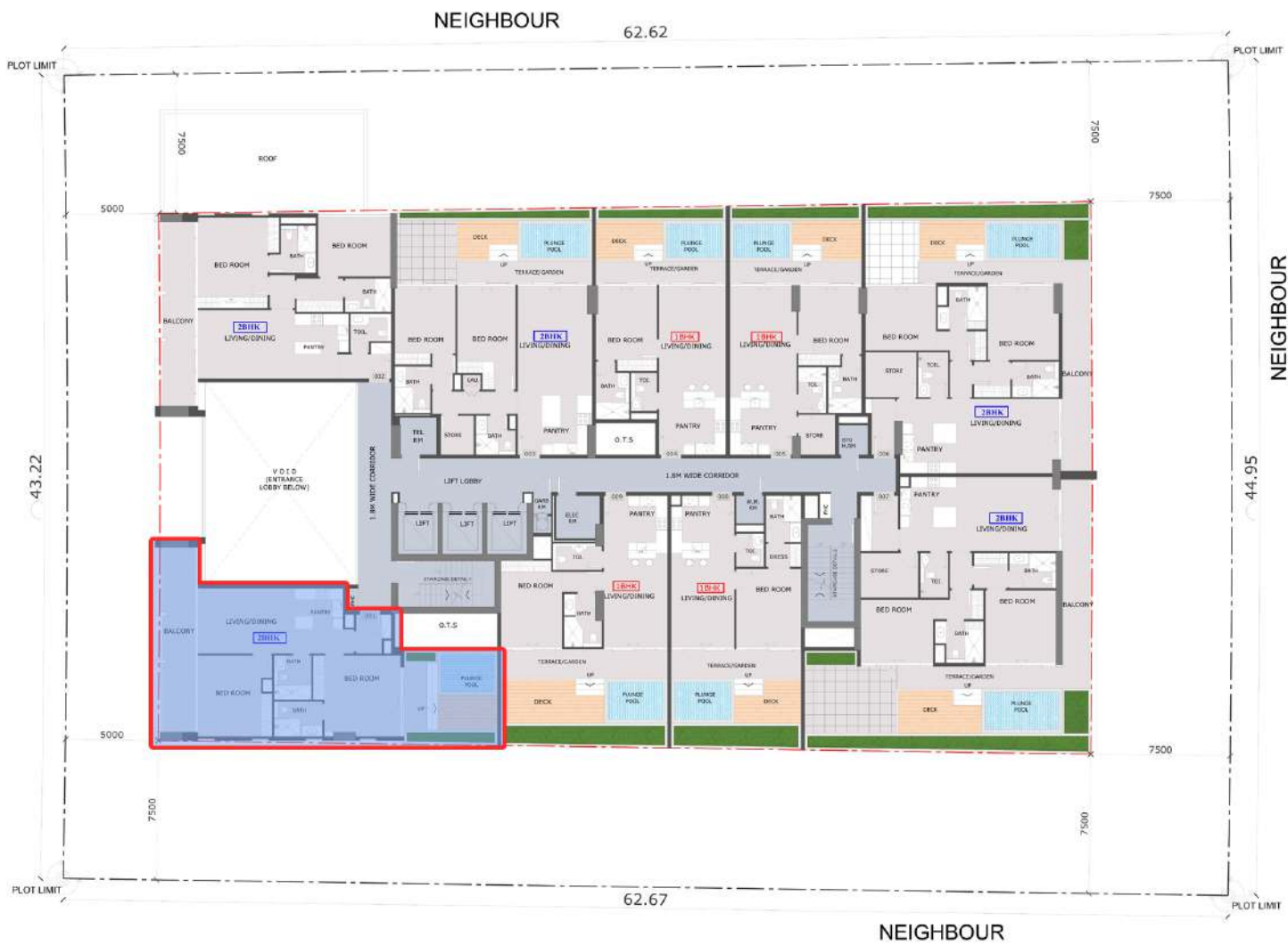
KEY PLAN
