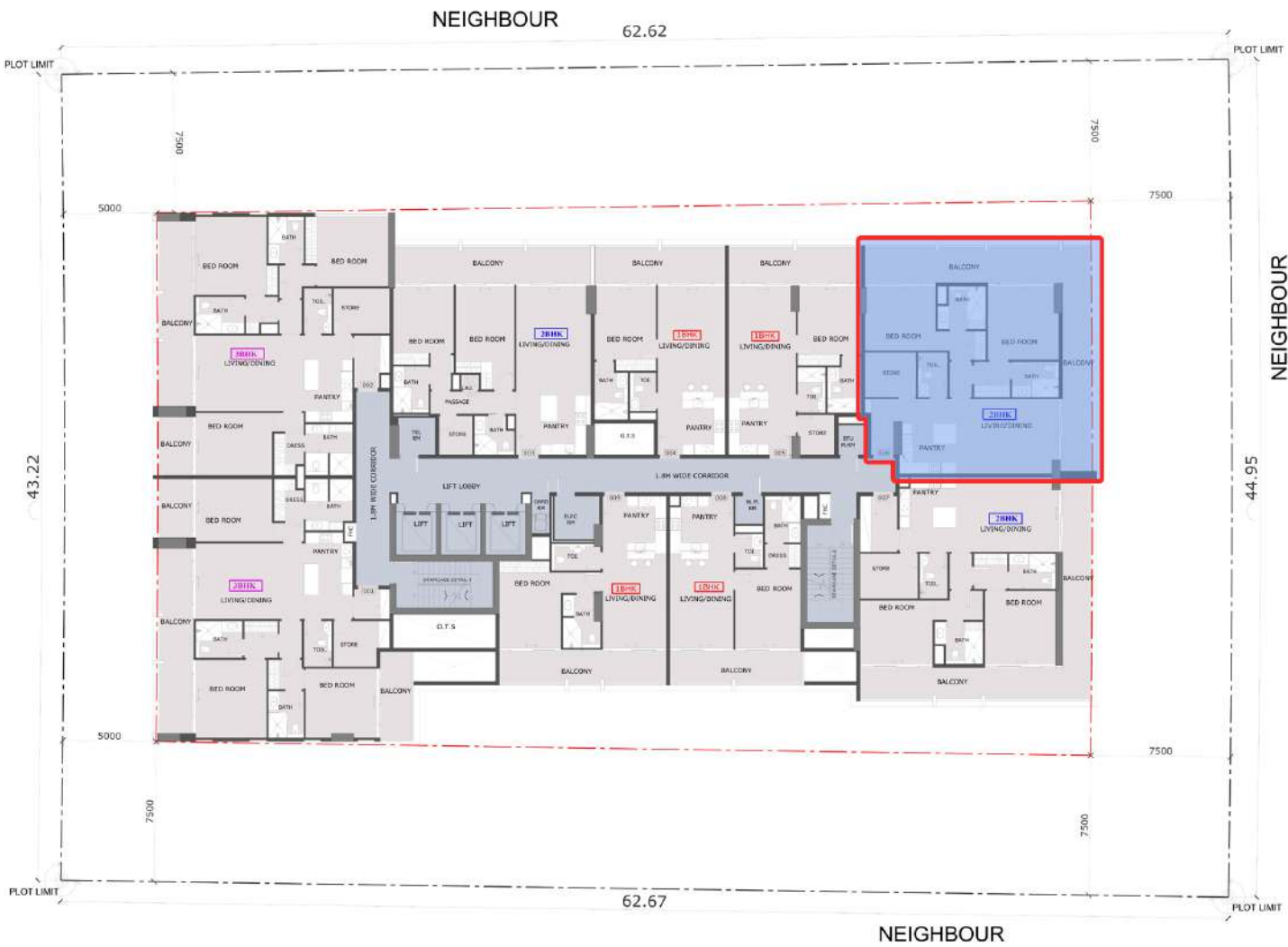
KEY PLAN
