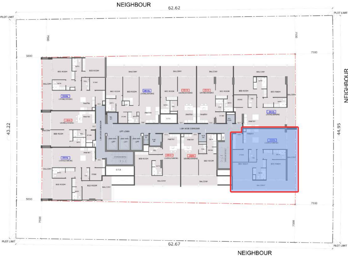
KEY PLAN
