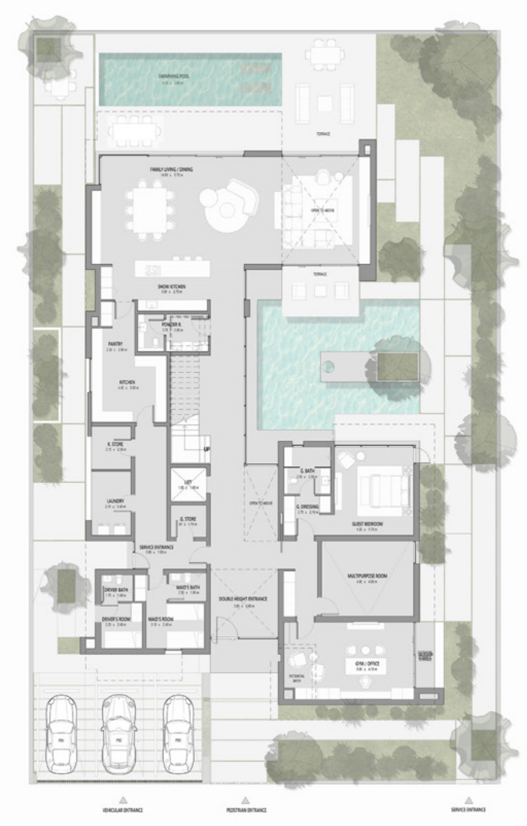
Ground Floor
