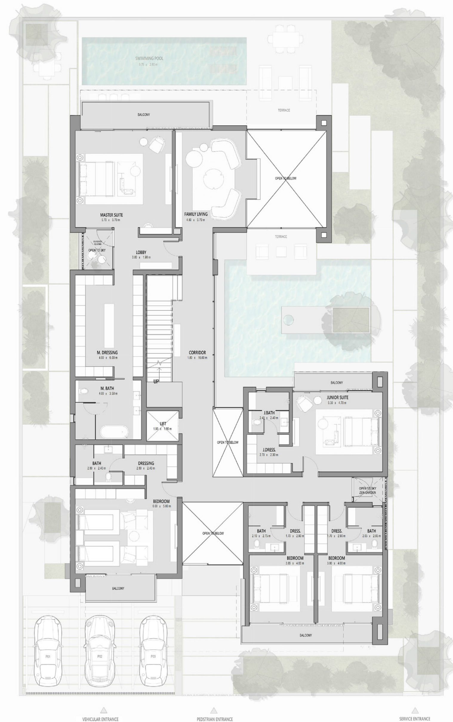
First Floor
