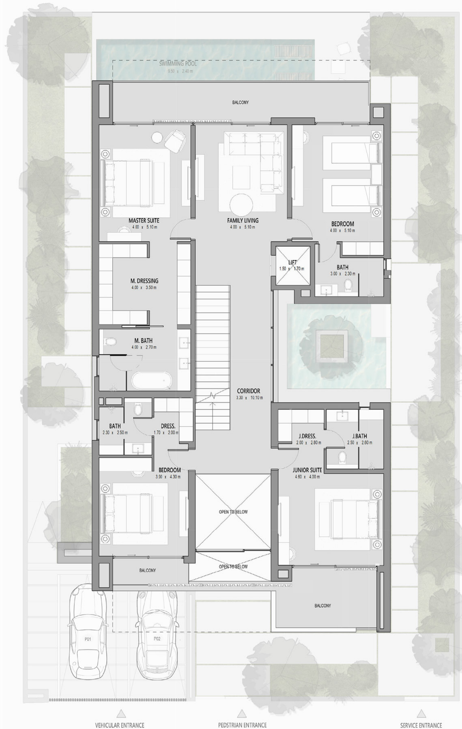
First Floor
