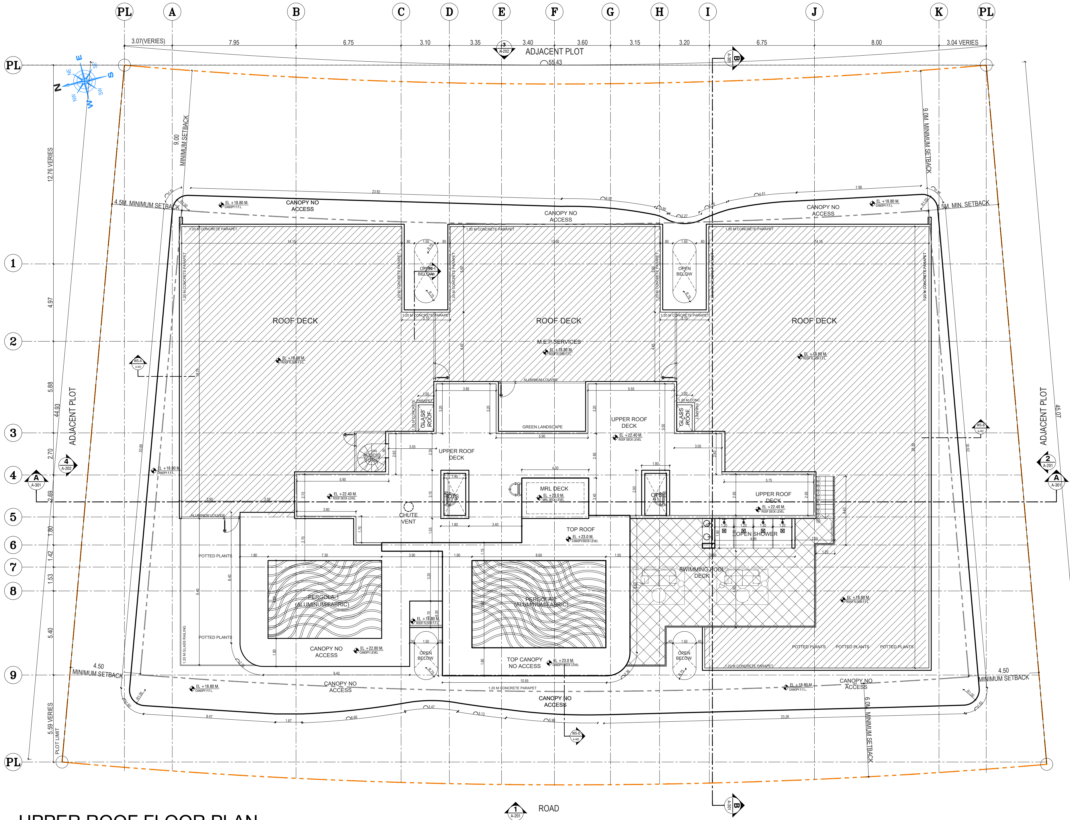
UPPER ROOF FLOOR PLAN
